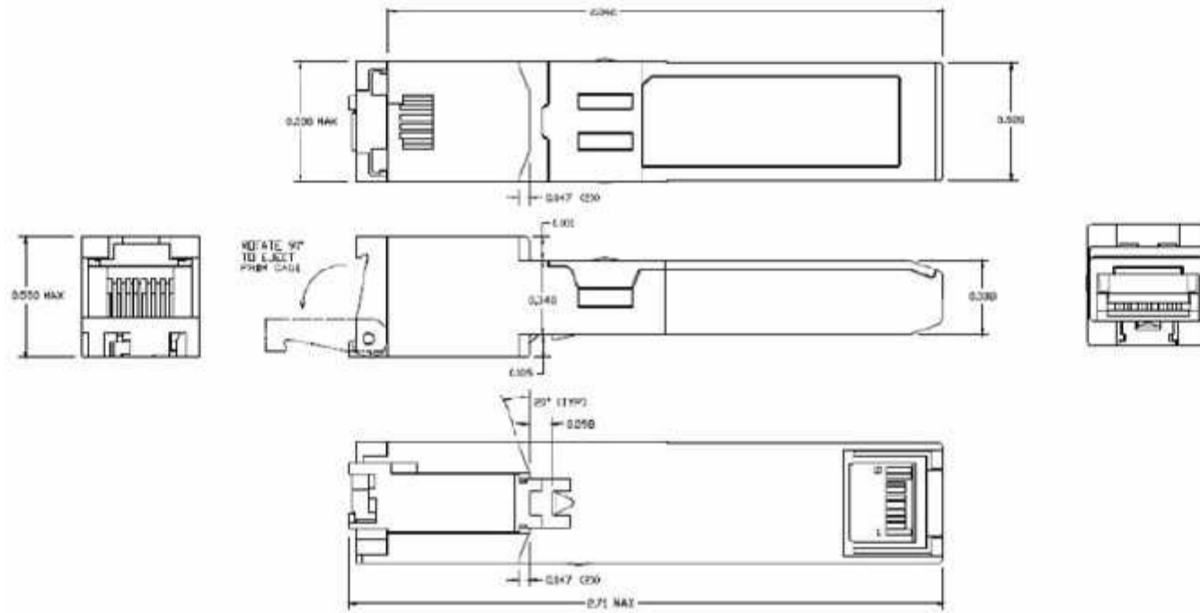
Figure 2. AP-STx mechanical dimensions
